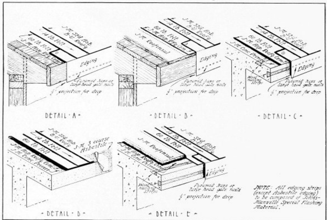
Details of Edging Strips in connection with Johns-Manville Standard Asbestos Built-up Roofing—Drawing F-31
