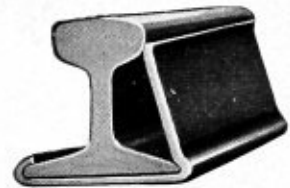
Transmission rail of the Elevated and the New York Subway. The exposed parts covered by indurated fibre material.
