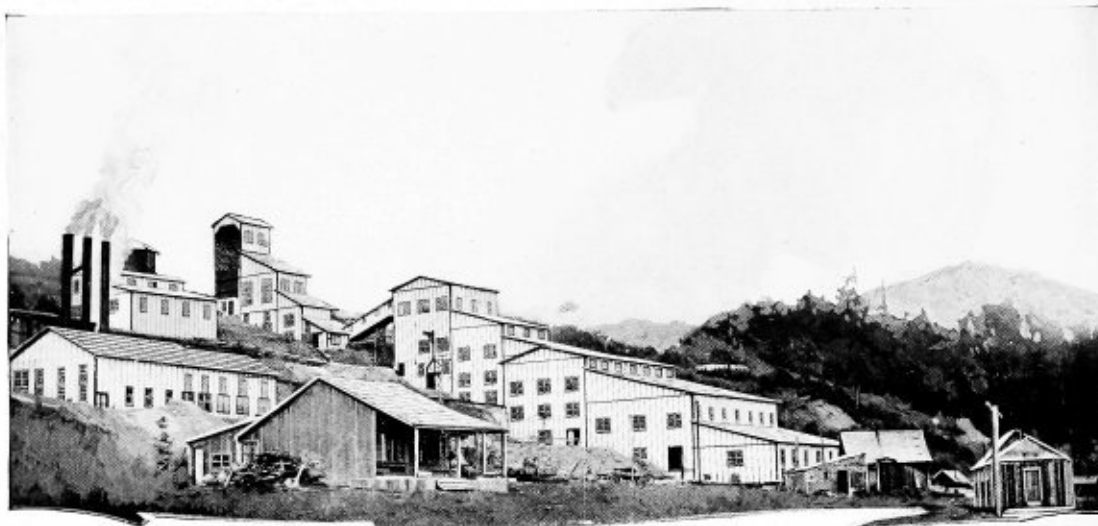
Washington Power and Reduction Co., Republic, Wash., showing application of Asbestoside with batten strips placed over vertical joints.
