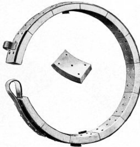
Showing Johns-Manville Asbesto-Metallic Friction Blocks applied to a brake band.
