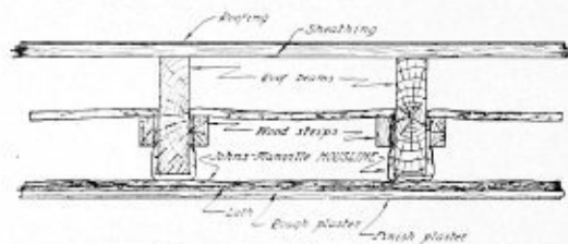
Housline under roof.
