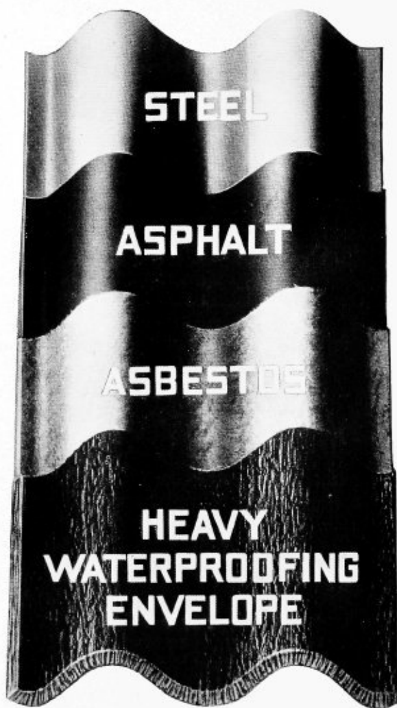
Sample of Asbestos Protected Metal with portions cut away to show relative position of the three corrosion-proof and insulating coatings with steel base or core.
