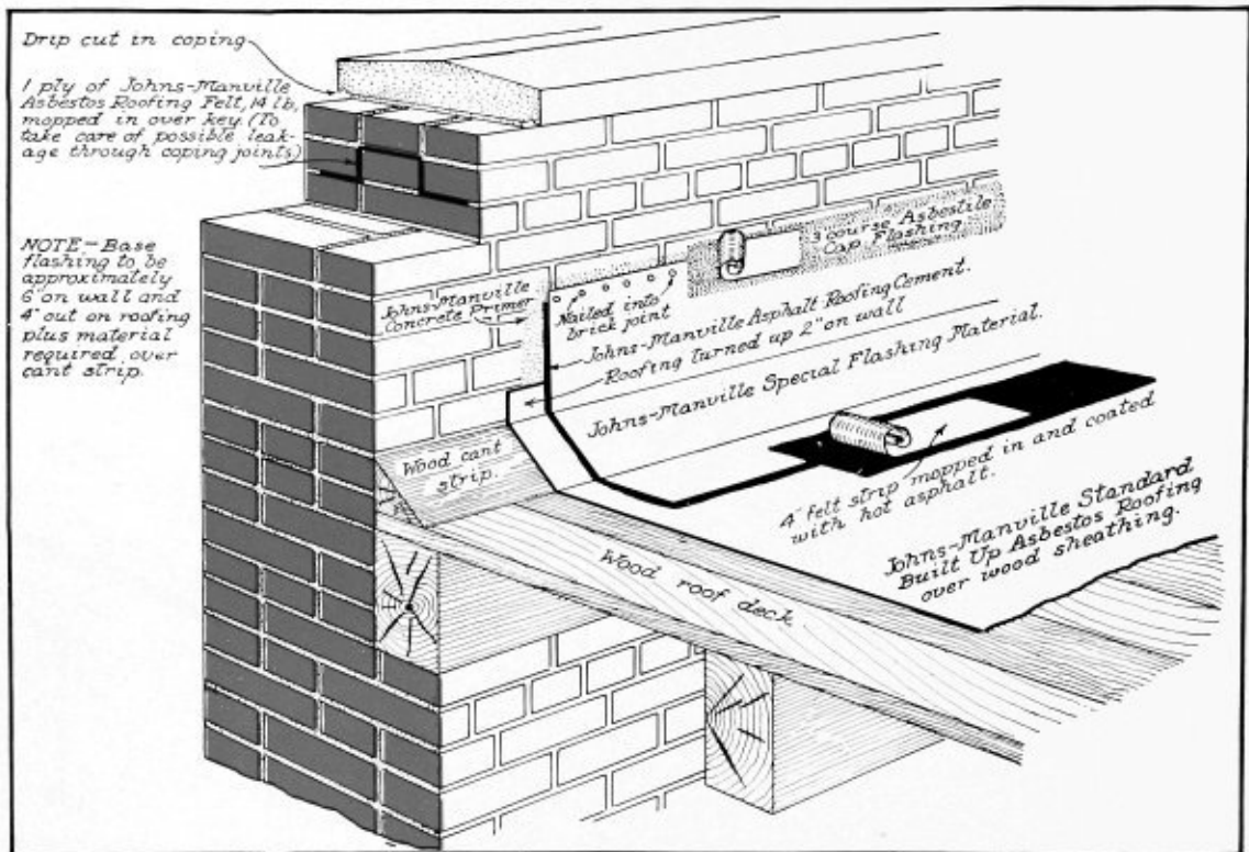
Details of Johns-Manville Asbestile System of Flashing. (Brick wall and wood deck)—Drawing F-28.
