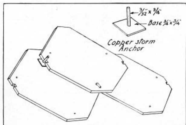
Hexagonal Shingle—Showing Application of Storm Anchor. Enlarged Scale.
