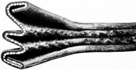
Cross-section of Coil Style No. 33, end opened to show construction.
