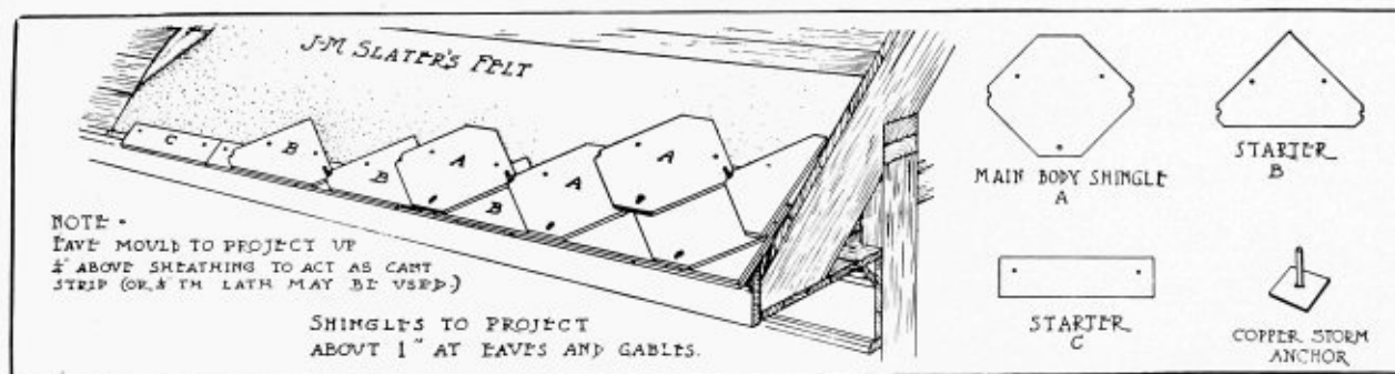
Sketch showing application of Johns-Manville Asbestos Shingles, Hexagonal Method.
