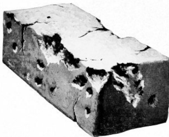
This illustration shows how severe heat attacks and destroys fire brick when it is not properly protected by carefully chosen refractories. Surface cracking and spawling and the expense of consequent shut downs and replacements, can be reduced by bonding and wash-coating fire brick with Johns-Manville refractories.
