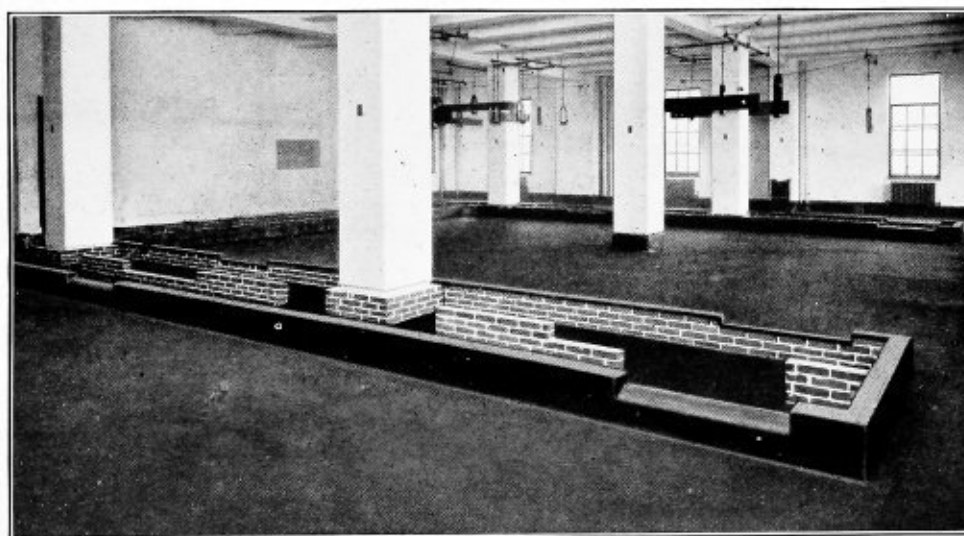
Typical installation of Acid-resisting Industrial Flooring in the battery room of the Triangle Exchange, New York Telephone Company, Brooklyn, N. Y.
