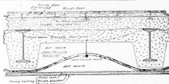
Housline in suspended ceiling.
