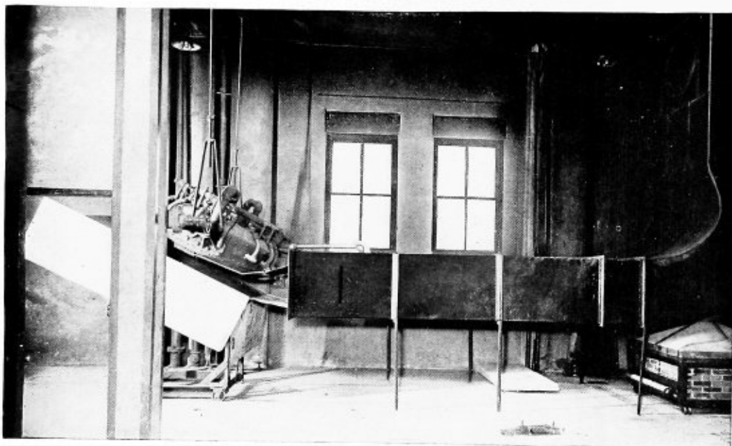
FIG. 2—APPARATUS USED IN MAKING STANDARD FIRE TESTS OF ROOF COVERINGS
