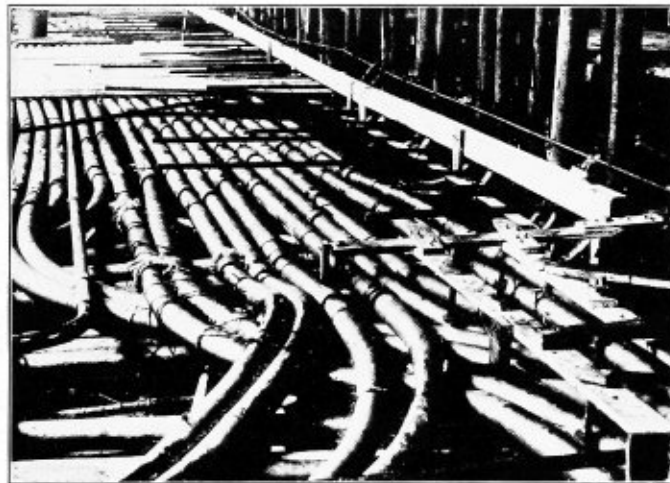
Installation of Fibre Conduit, Switchboard Floor, between lines "E" and "F", at United Electric Company, Springfield, Mass., Stone and Webster, Inc., Engineers and Contractors.
