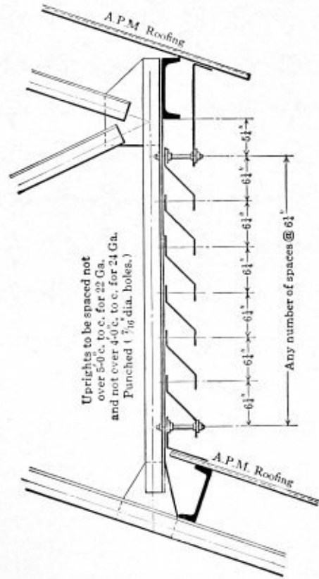
LOUVER TYPE B CONSTRUCTION
