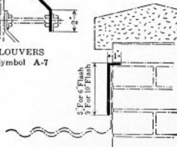
COUNTER FLASHING Symbol A-6
