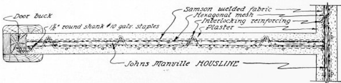
Housline in Samson Sound-proof Partition.
