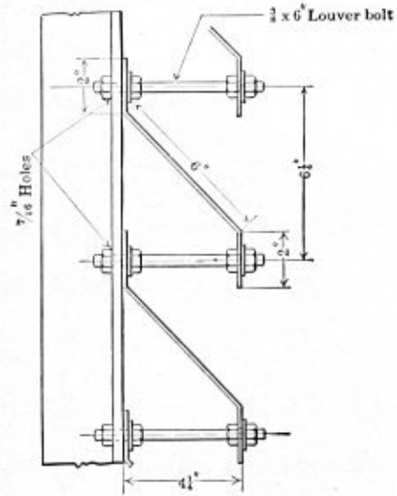
LOUVER TYPE B CONSTRUCTION
