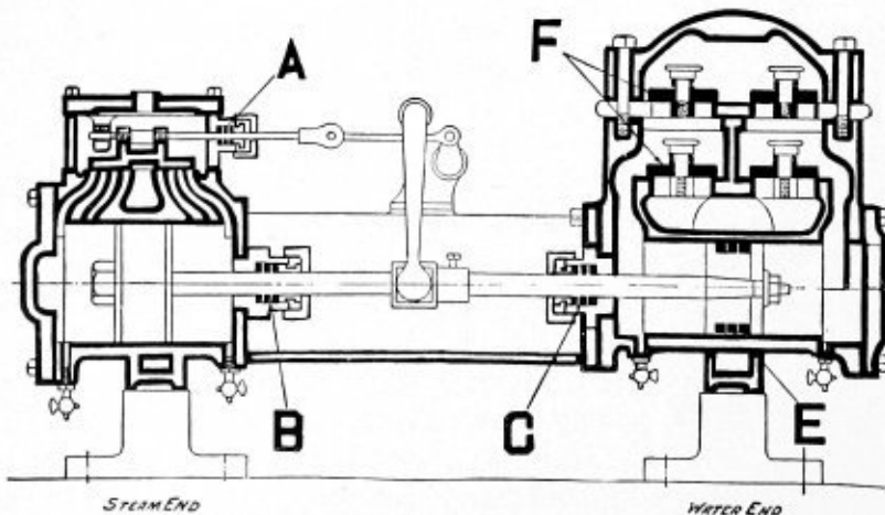
Inside Packed Type of Pump.
