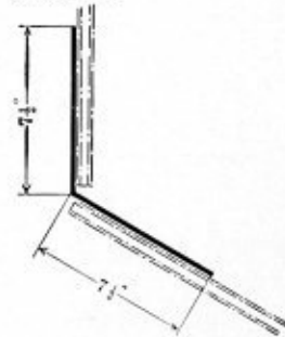
END WALL FLASHING Symbol A-4
