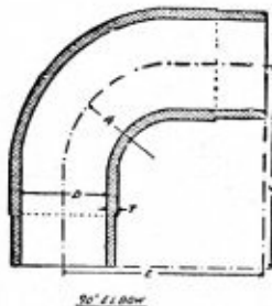
90° ELBOW
