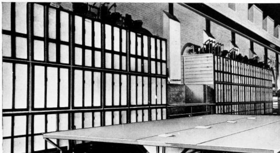
Oil switch compartments and transformer protective cover of Transite Asbestos Wood. Installed at Station F, Pacific Gas and Electric Co., San Francisco, Calif.
