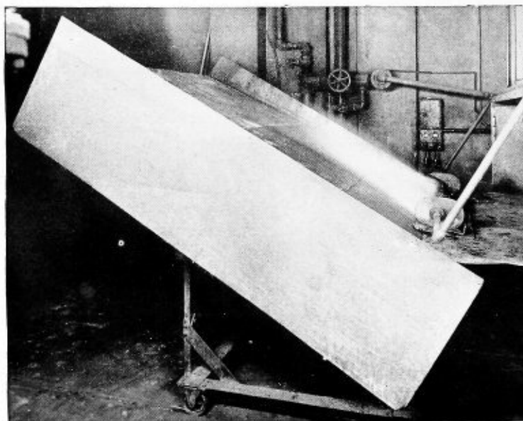
Fig. 7—Flame Exposure Test Apparatus in Action. See pages 106 and 109 for details.
