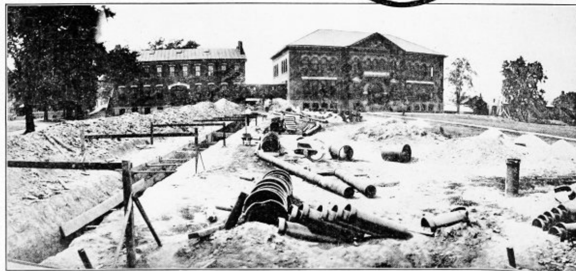
Sections being split before being placed in trench at Pennsylvania Reform School, Morgantown, Pa.
