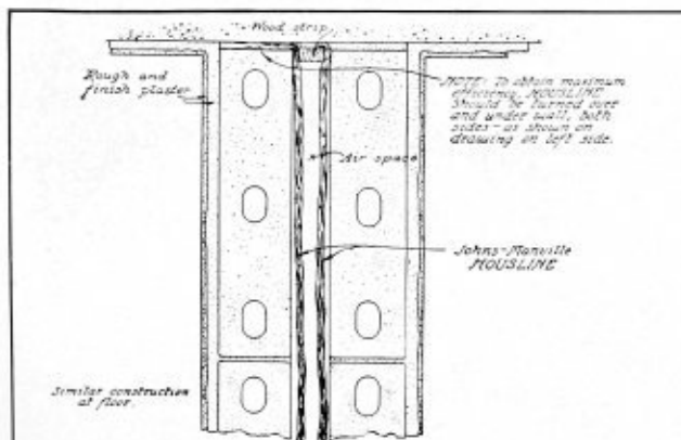
Section through partition, Gypsum Blocks or Hollow Tile.
