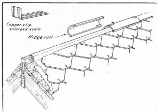
Hexagonal Shingle on roof.
