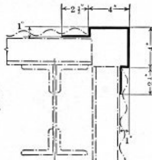
CORNER TRIM Symbol A-2
