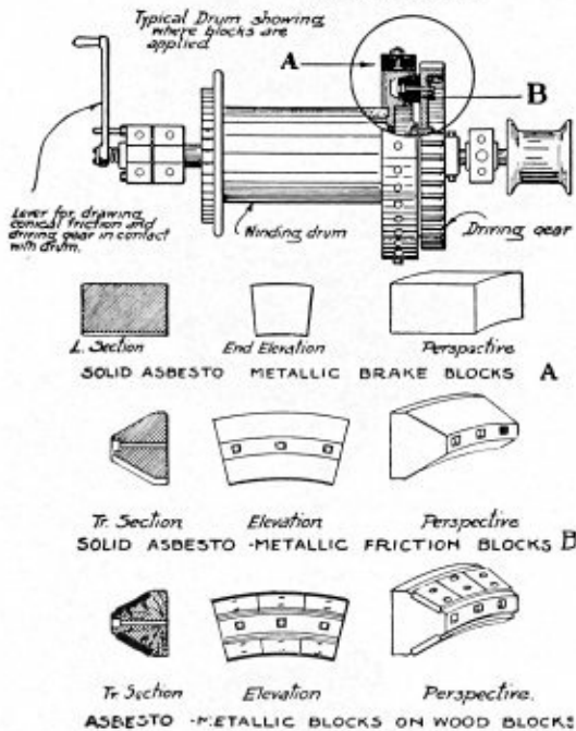
HOISTING DRUM EQUIPPED WITH FRICTION AND BRAKE BLOCKS
