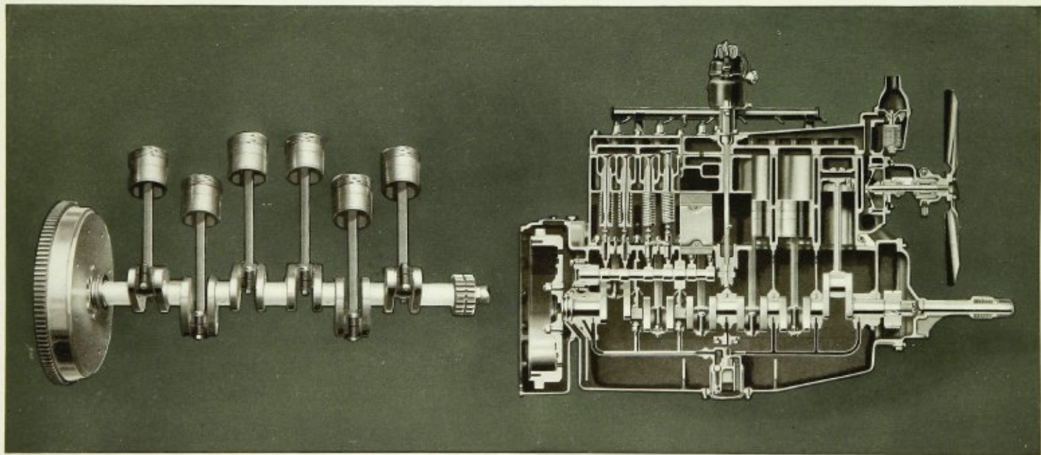
SINGLE-SIX CRANKSHAFT—Shows the seven main bearings and machined all over surfaces. Perfectly balanced and contributing greatly to freedom from motor vibration.
