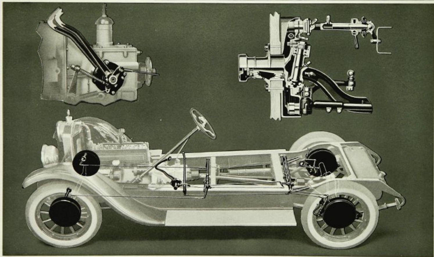
PLANETARY STEP-UP GEAR—Affords maximum in braking pressure with minimum of pedal travel and effort.
