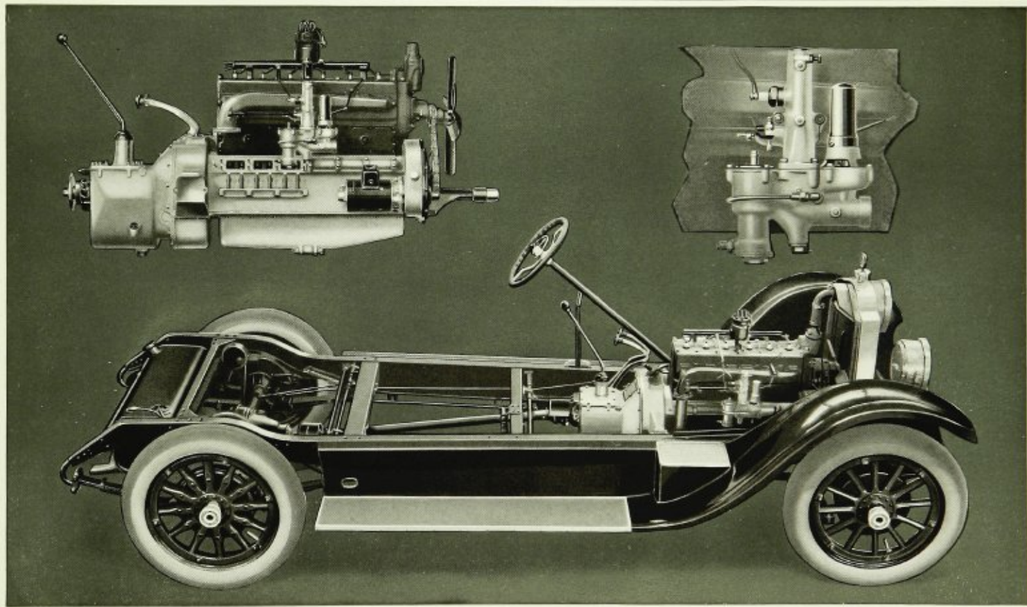
SINGLE-SIX MOTOR—The Single-Six motor, Packard in design and construction, affords ample power with a minimum of fuel and oil consumption.
