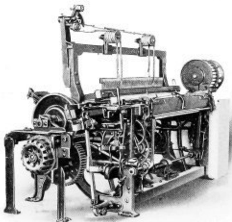
NORTHROP LOOM AS EXHIBITED AT PHILADELPHIA.
