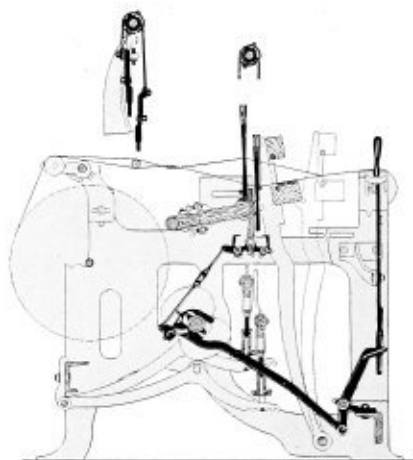
DOUBLE STEEL HARNESS.
