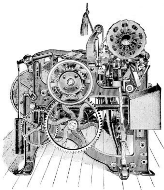
END VIEW OF A MODEL LOOM.
