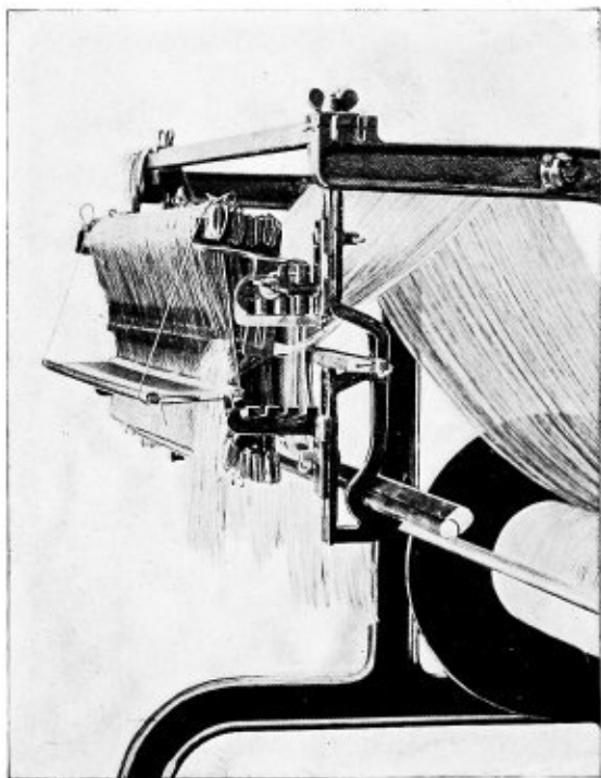
THE KEENE DRAWING-IN FRAME.
