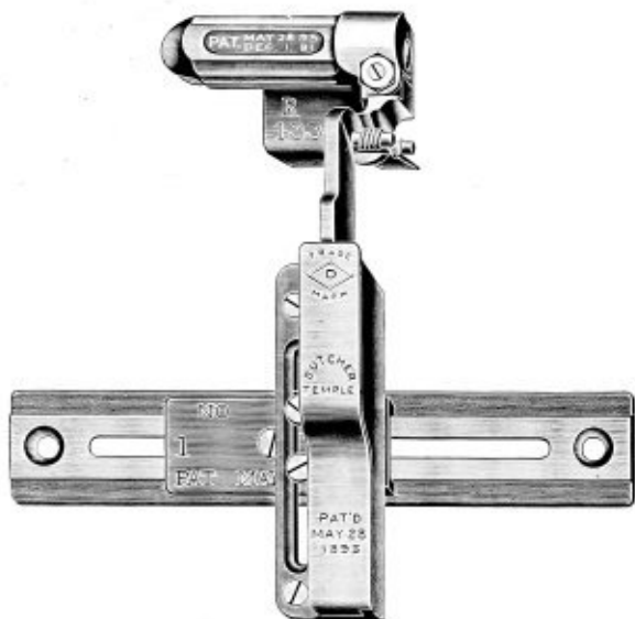
LATEST FORM OF THREAD-CUTTING TEMPLE. NUMBER 133.
