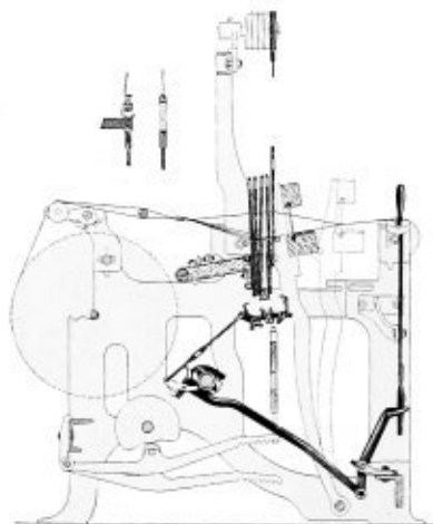
MULTIPLE STEEL HARNESS.
