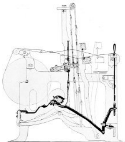
DOUBLE THREAD DROPS.
