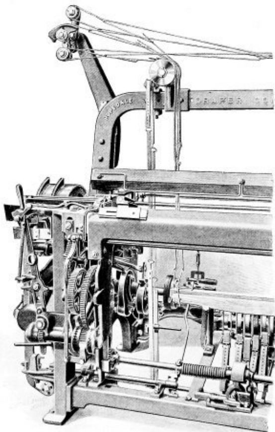
DETAIL OF LACEY TOP-RIG ON D MODEL.
