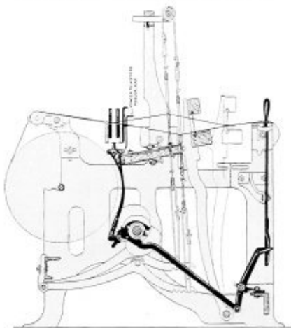
LEASING DROP WIRES.
